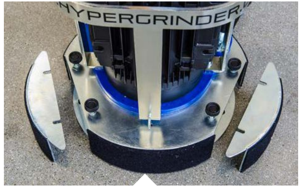
The quick release covers allows a speedy conversion to wall grinding on two sides.
