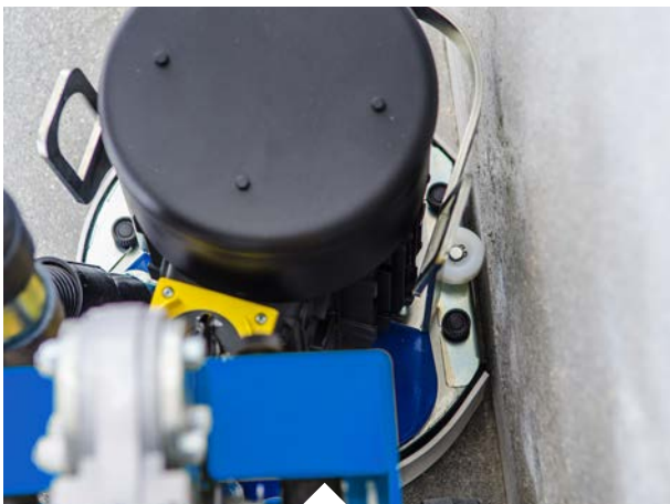
The guided wheel allows the optimal working position and facilitates the smoothing of the wall.
